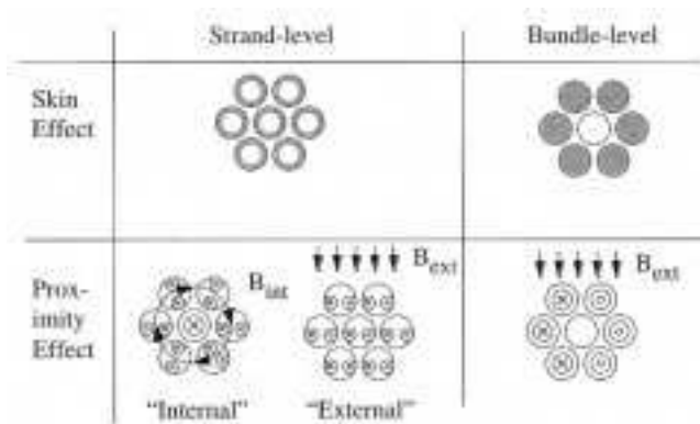
Fig. 1. Types of eddy-current effects in litz wire.
